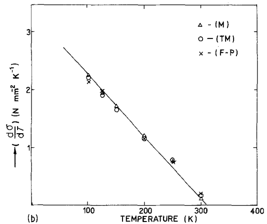
Figure 2 (a) The variation of yield stress of A-203D steel with temperature under various microstructural conditions. (b) Extrapolation of stress differential to zero to determine critical temperature, T_c , in A-203D steel.
